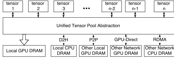
Figure 7: The unified tensor pool provides a consolidated memory abstraction to include various physical memory pools for tensor allocations.
